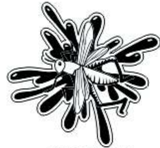
BUG SPLAT 2 File Name: ELB06.EPS
